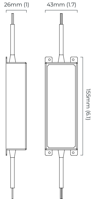
Remote LED Driver Dimensions
