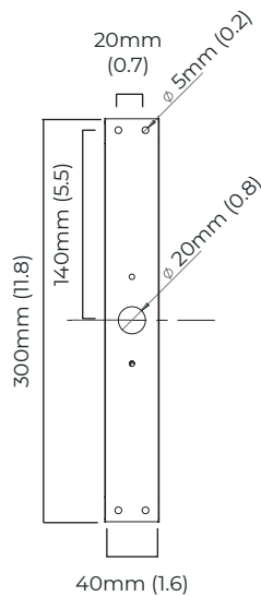
mounting plate dimensions
