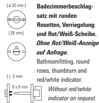
Drückerrosettenpaar, rund. Pair of lever roses, round.
